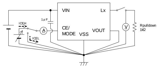
Circuit⑧
