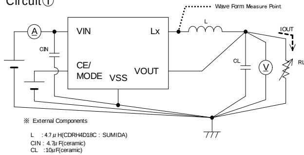
Circuit①
