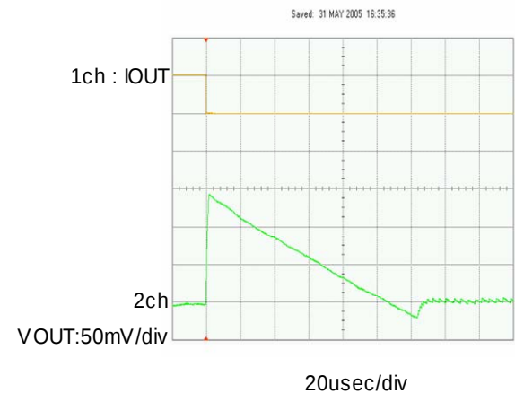
IOUT=300m A → 1m A
