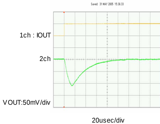
IOUT=1m A → 100m A
