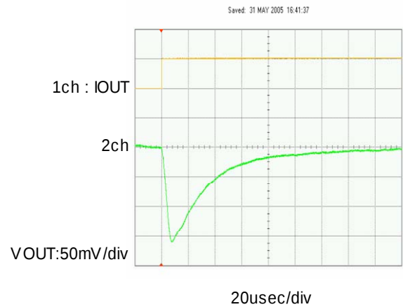
IOUT=1m A → 300m A
