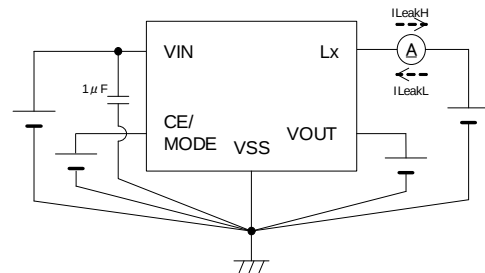
Circuit⑥
