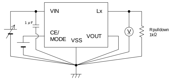
Circuit②
