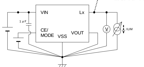
Circuit⑨
