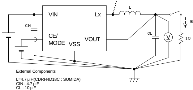
Circuit⑨
