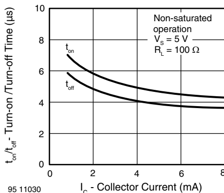
Fig. 13 - Turn-on/off Time vs. Collector Current
