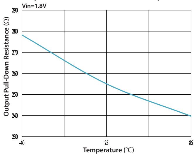
Output Pull-Down Resistance vs. Temperature
