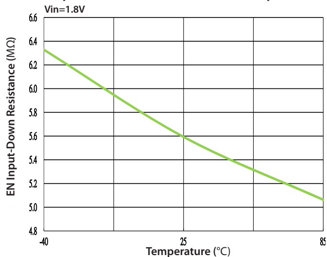
EN Input Pull-Down Resistance vs. Temperature
