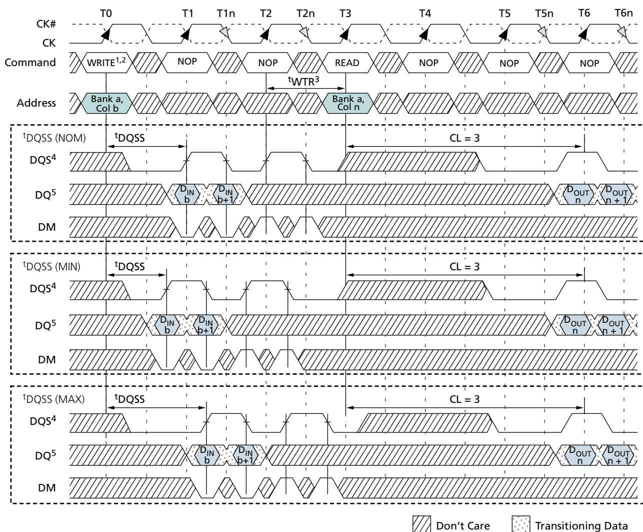
Figure 39: WRITE-to-READ – Interrupting
