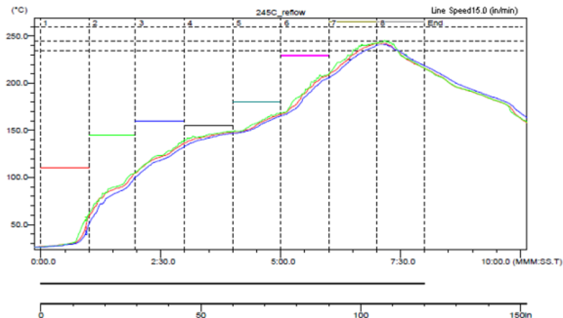
Figure 24. Sample Reflow Profile
