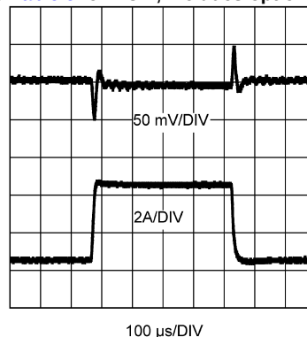
Load Transient Response V_{IN} = 5.0V , V_{OUT} = 2.5V , I_{OUT} = 0.5A to 4.5A to 0.5A step 20 MHz Bandwidth Limited Refer to Table 5 for BOM, includes optional components
