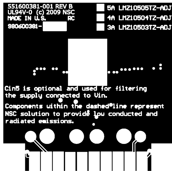
Figure 29. Bottom Copper
