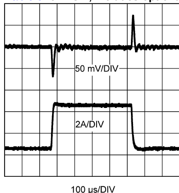
Load Transient Response V_{IN} = 3.3V , V_{OUT} = 2.5V , I_{OUT} = 0.5A to 4.5A to 0.5A step 20 MHz Bandwidth Limited Refer to Table 5 for BOM, includes optional components
