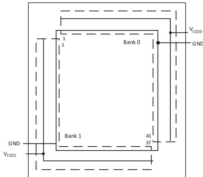
Figure 2.21. MachXO256 Banks
