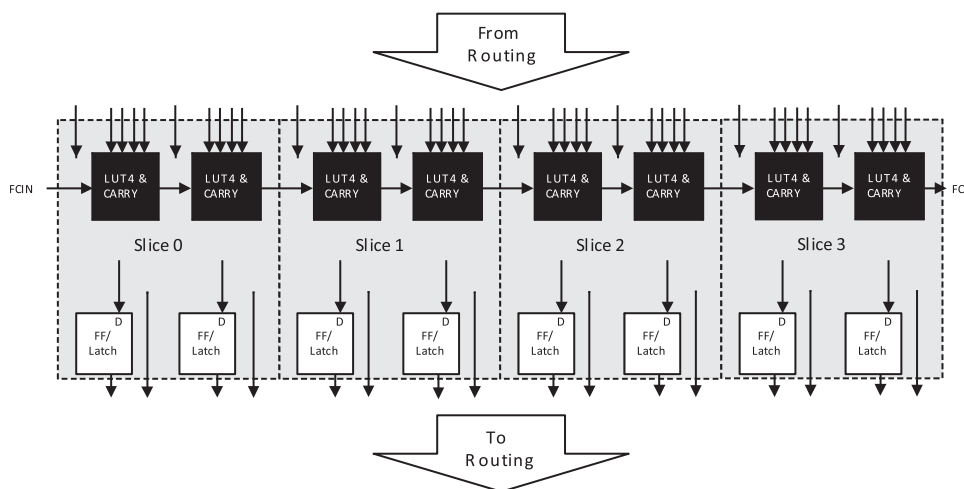
Figure 2.4. PFU Diagram
