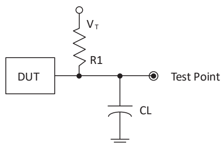
Figure 3.6. Output Test Load, LVTTTL and LVCMOS Standards
