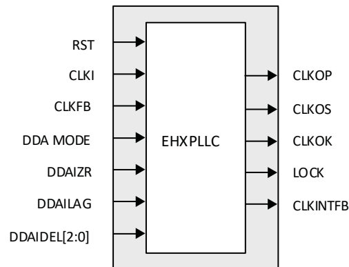
Figure 2.11. PLL Primitive
