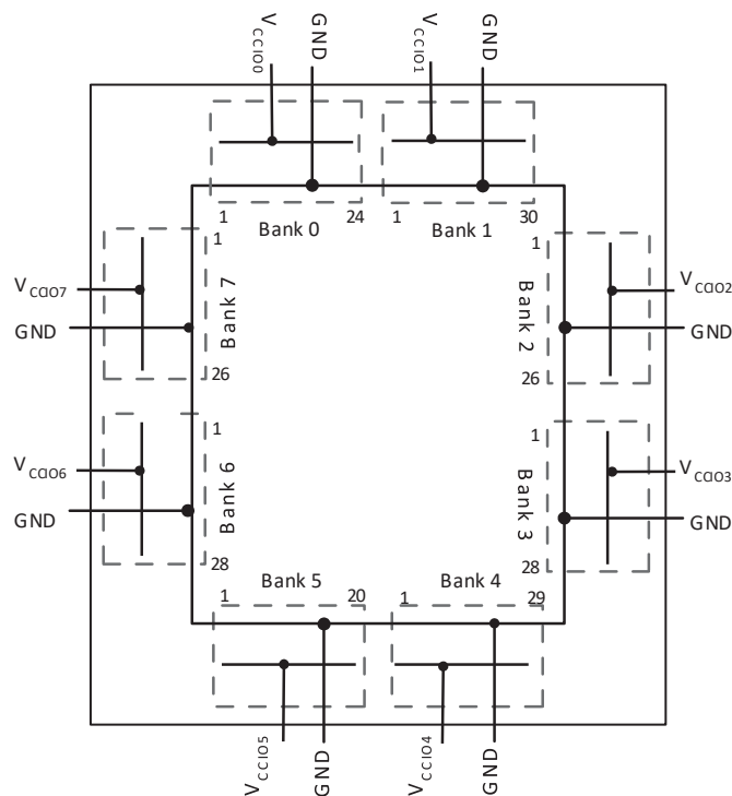
Figure 2.19. MachXO1200 Banks
