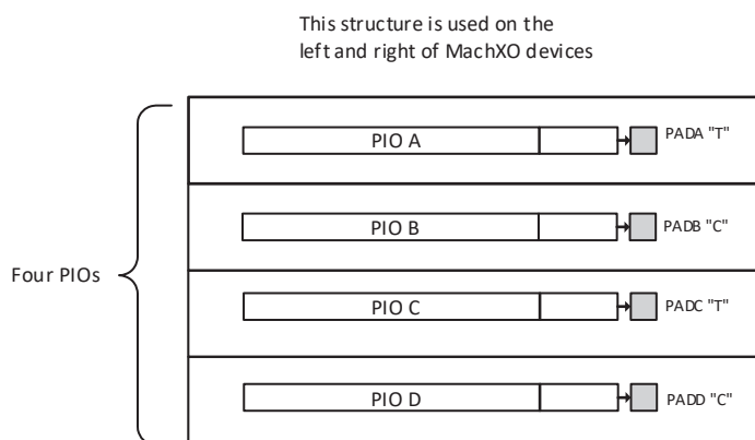
Figure 2.15. Group of Four Programmable I/O Cells
