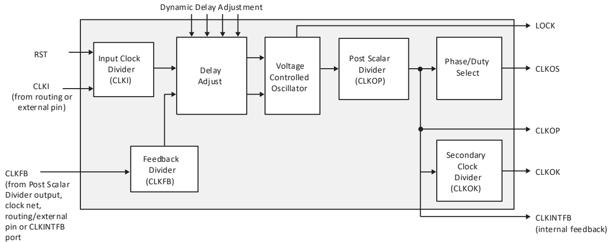
Figure 2.10. PLL Diagram
