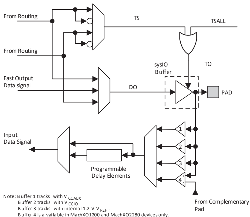
Figure 2.17. MachXO PIO Block Diagram
