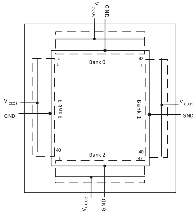
Figure 2.20. MachXO640 Banks
