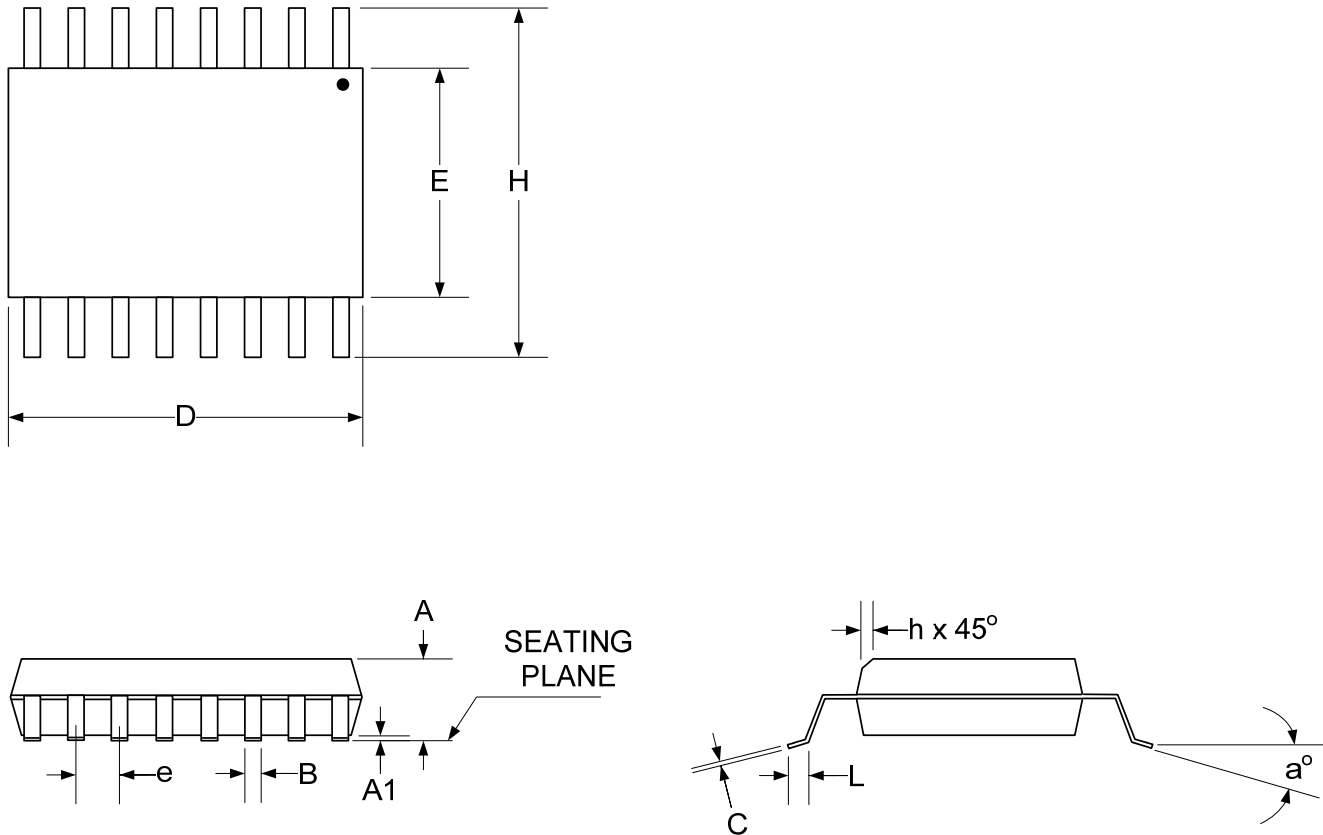
Figure 10 – 16-Pin QSOP (150 Mil) Dimensions
