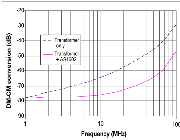
Figure 4 – DM-CM Conversion in Receiving Data from UTP with Typical 2-Core PoE Compatible Transformers using 3-Wire PHY-Side Choke
