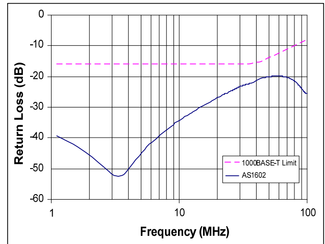
Figure 5 – AS1602 Return Loss with Typical 3-Core PoE Compatible Transformer with Media Side Chokes
