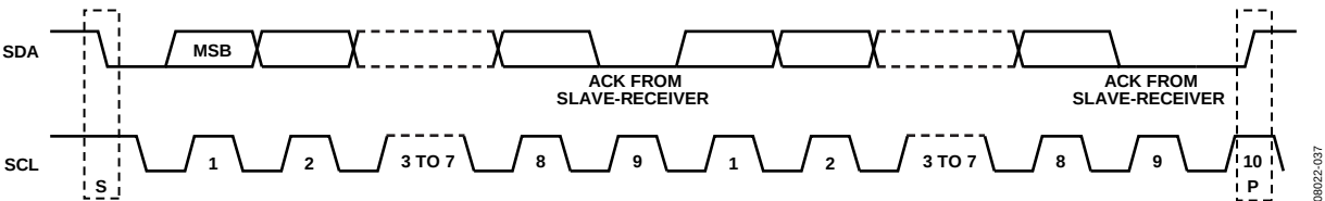
Figure 64. Acknowledge Bit
