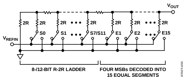
Figure 37. DAC Ladder Structure
