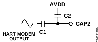
Figure 42. Coupling HART Signal
