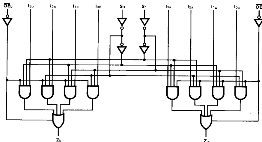
LOGIC DIAGRAM
