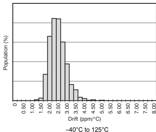
Figure 6-2. Temperature Drift
