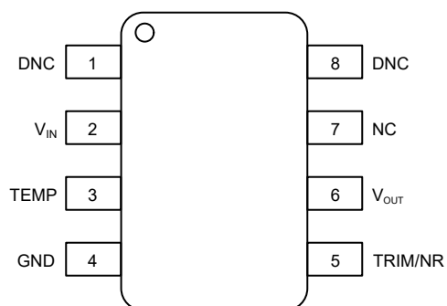
Figure 5-1. REF50xxAI, REF50xxI 8-Pin SOIC, VSSOP Top View
