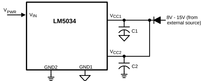
Figure 31. External Power to V_{CC}
