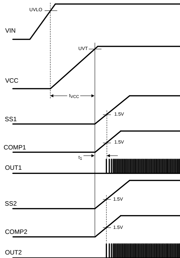
Figure 5. Startup Sequence
