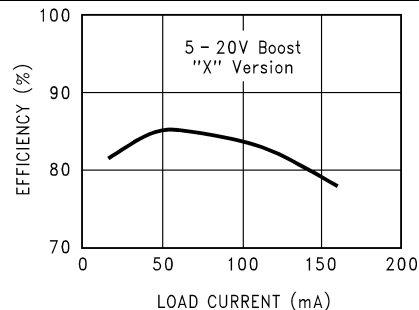
Figure 32. Efficiency vs. Load Current (5-20V X-version)
