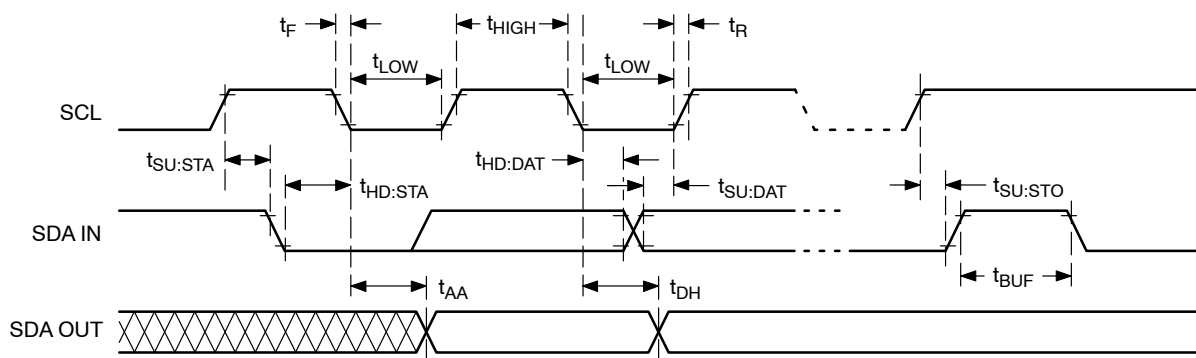
Figure 5. Bus Timing
