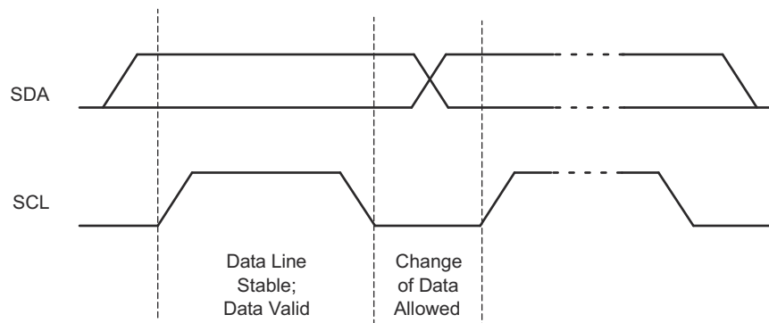
Figure 8-4. Bit Transfer
