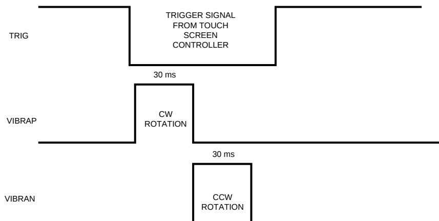
Figure 31. Control Waveform
