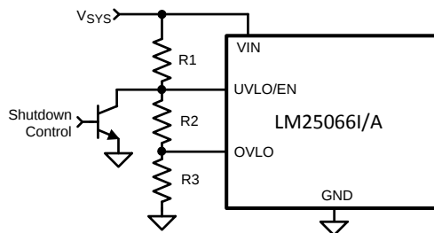
Figure 35. Shutdown Control
