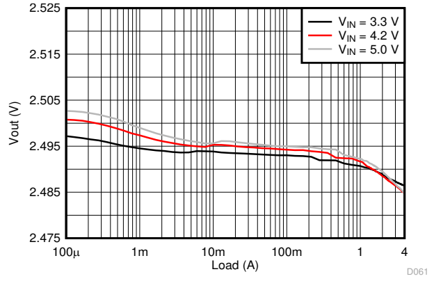
Figure 9-16. Load Regulation
