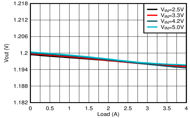
V OUT = 1.2 V F-PWM devices Figure 9-10. Load Regulation
