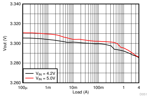
Figure 9-20. Load Regulation
