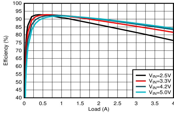
V OUT = 1.2 V F-PWM devices Figure 9-9. PWM Efficiency
