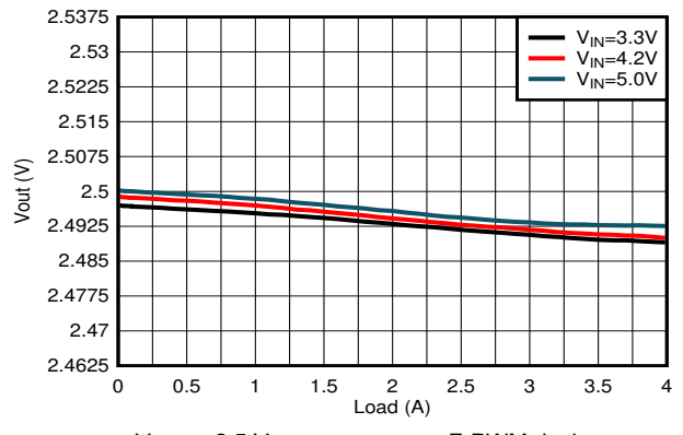
Figure 9-18. Load Regulation F-PWM devices
