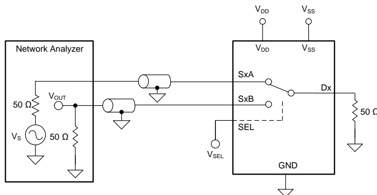
Figure 24. Intra-channel Crosstalk Measurement Setup
