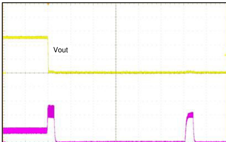
Figure 8-4. Hiccup Operation
