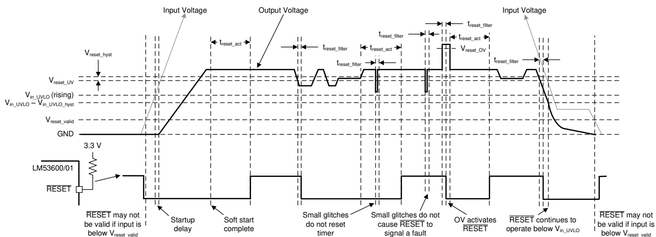
Figure 8-5. Reset Output Function Operation
