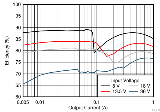
Figure 9-14. Efficiency
