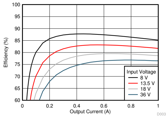
Figure 9-13. Efficiency
