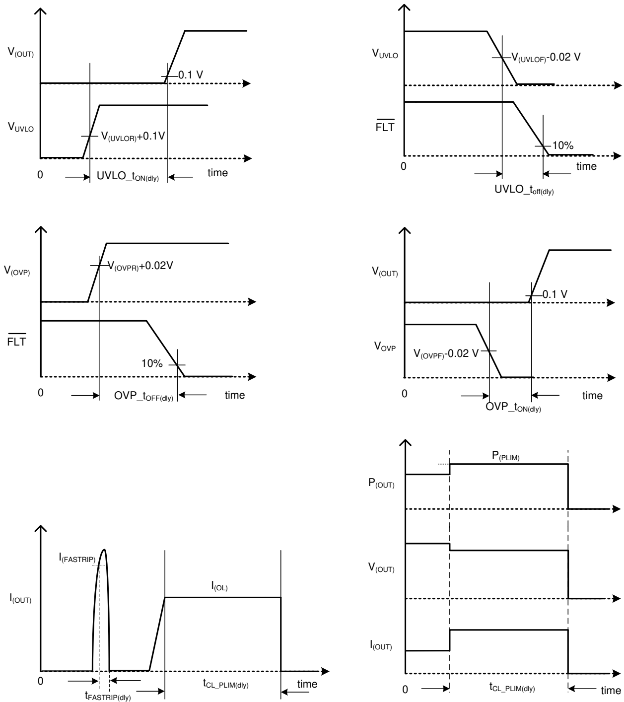
Figure 14. Timing Waveforms
