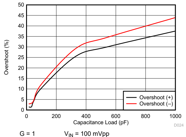
Figure 7-24. Small Signal Overshoot vs Capacitive Load
