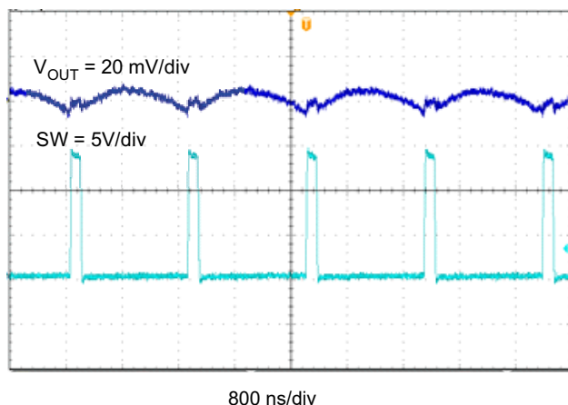
Figure 8-10. TPS562208 Output Voltage Ripple, I_{OUT} = 0 A
