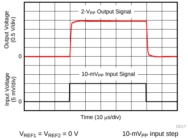
Figure 20. Step Response
