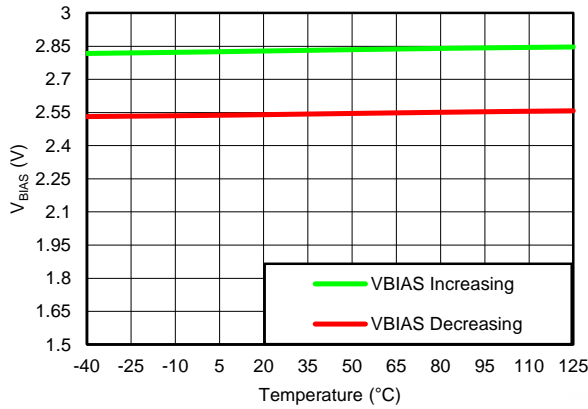
Figure 31. Minimum ANY-OUT V_{OUT} , Minimum V_{IN} BIAS UVLO Threshold vs Temperature
