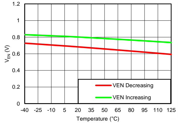
Figure 32. Minimum ANY-OUT V_{OUT} , Minimum V_{IN} , No BIAS Enable Threshold vs Temperature
