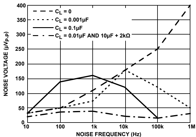
FIGURE 117. NOISE REDUCTION
