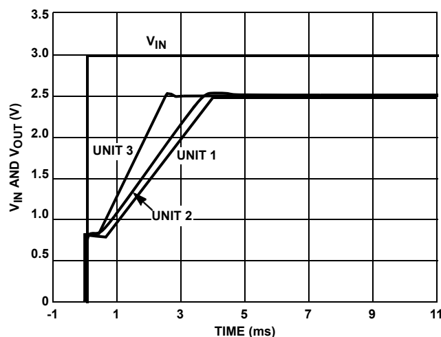
FIGURE 119. TURN-ON TIME
