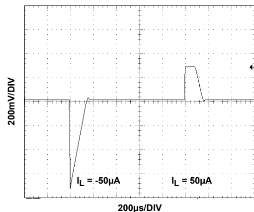
FIGURE 92. LOAD TRANSIENT RESPONSE
