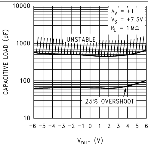
Figure 55. Stability vs Capacitive Load
