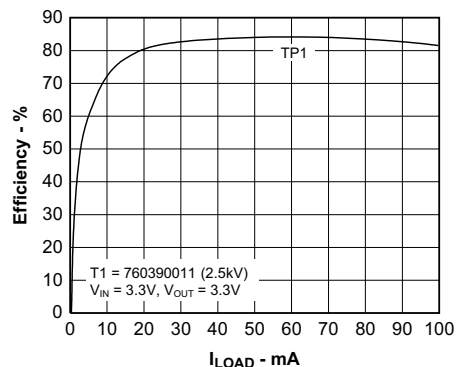
Figure 5-2. Efficiency vs Load Current
