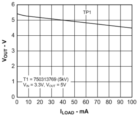
Figure 5-19. Output Voltage vs Load Current
