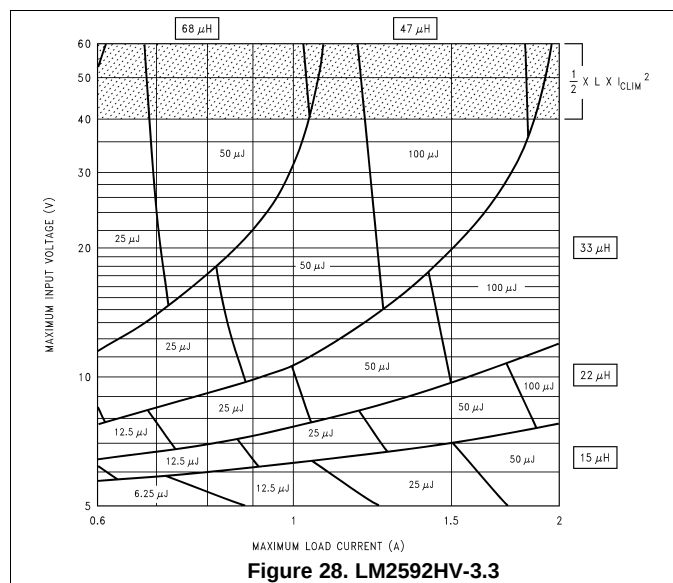
Figure 28. LM2592HV-3.3
