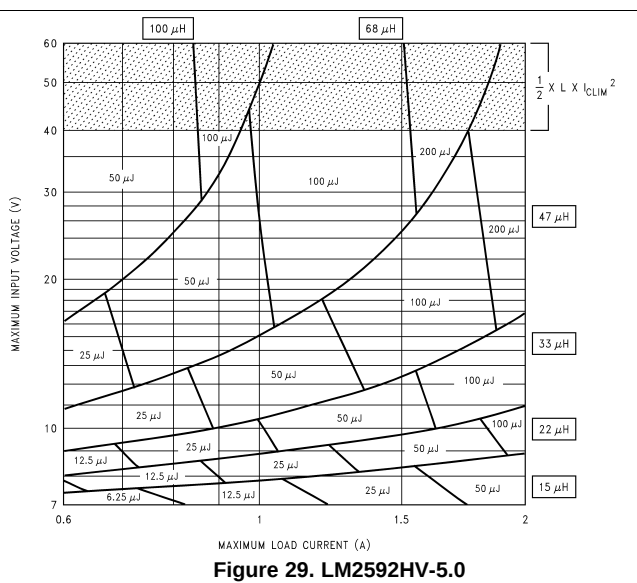
Figure 29. LM2592HV-5.0
