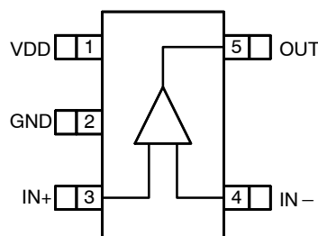
SOT23-5 (Top View)
