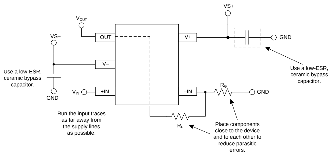
Figure 49. Layout Example
