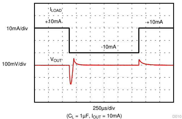
Figure 7-12. Load Transient
