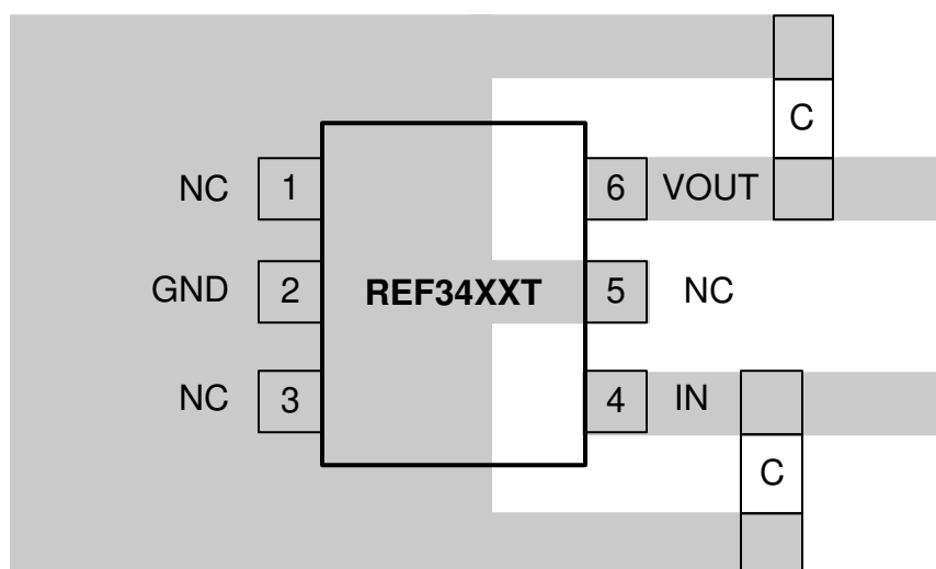
Figure 12-2. REF34xxT Layout Example
