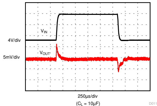
Figure 7-15. Line Transient
