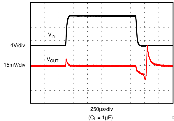
Figure 7-14. Line Transient
