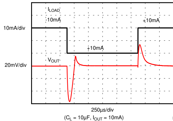
Figure 7-13. Load Transient
