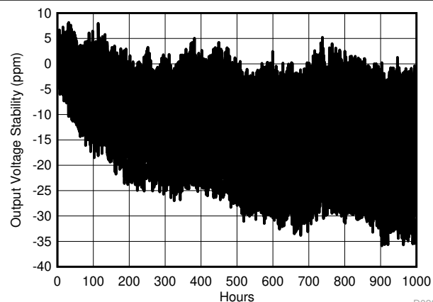
Figure 7-22. Long Term Stability - 1000 hours ( V_{OUT} )
