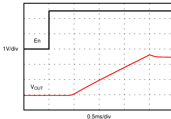
Figure 7-20. Turnon Time (Enable)
