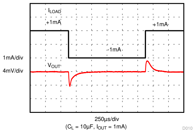
Figure 7-11. Load Transient
