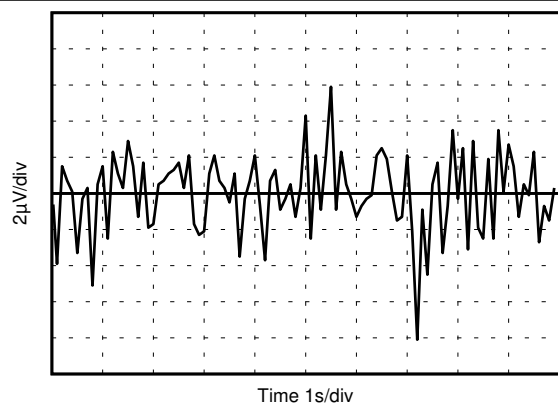
Figure 7-21. 0.1-Hz to 10-Hz Noise ( V_{OUT} )
