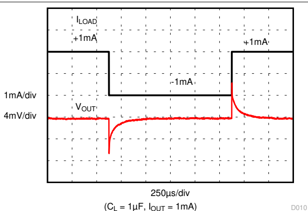
Figure 7-10. Load Transient
