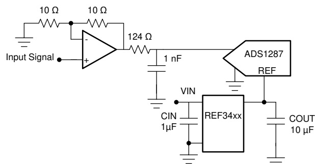
Simplified Schematic
