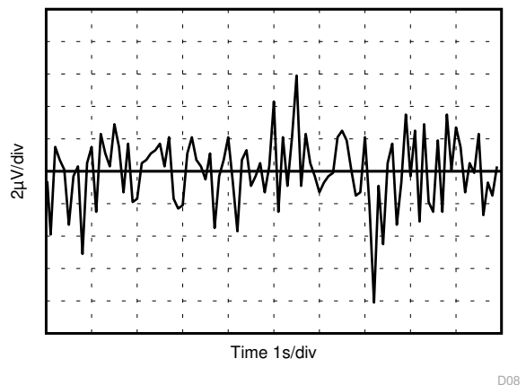
Figure 8-5. 0.1-Hz to 10-Hz Noise ( V_{OUT} )
