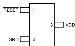
Figure 6-2. TLV853: DBZ Package 3-Pin SOT-23 Top View
