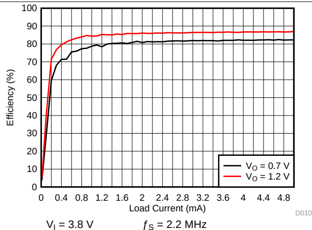
Figure 4-4. SMPS Efficiency for Multi-Phase Eco-mode
