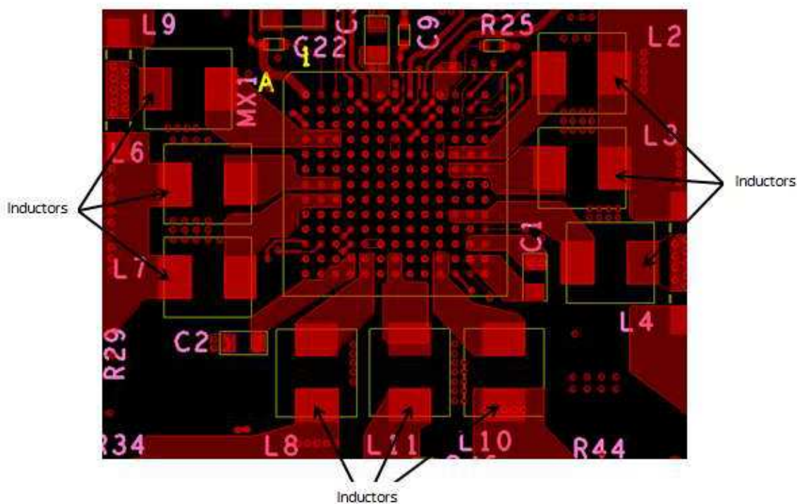
Figure 8-4. Top-Layer Overview of Inductor Placement
