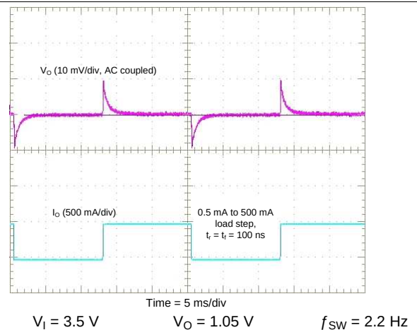
Figure 6-14. Typical SMPS Load Transient Response for SMPS12, SMPS3, SMPS45, SMPS6, and SMPS7
