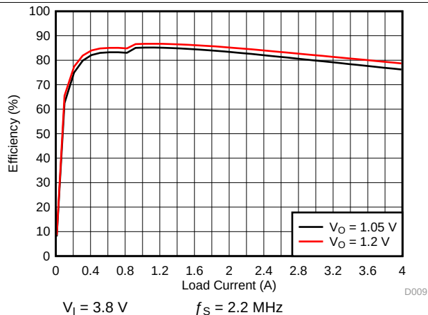
Figure 4-5. SMPS Efficiency for 4-A Multi-Phase PWM Mode
