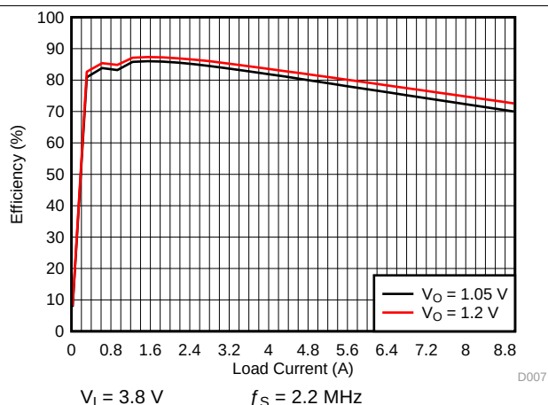
Figure 4-7. SMPS Efficiency for 9-A Multi-Phase PWM Mode
