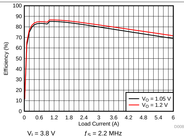
Figure 4-6. SMPS Efficiency for 6-A Multi-Phase PWM Mode
