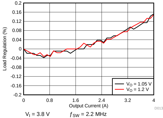
Figure 6-9. SMPS Load Regulation for 4-A Dual Phase
