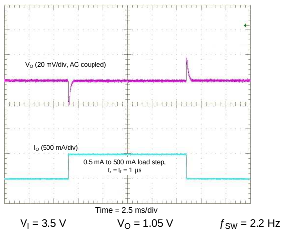
Figure 6-13. Typical SMPS Load Transient Response for SMPS8 and SMPS9
