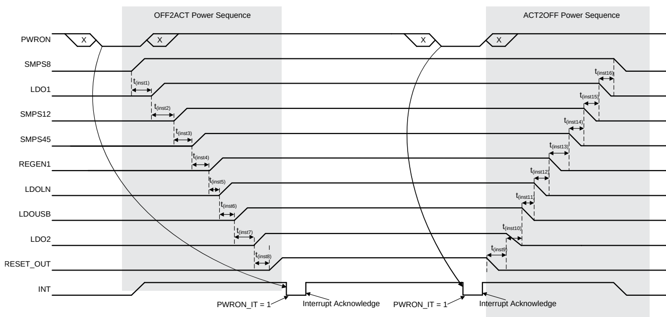
Figure 5-19. Power Sequence Example
