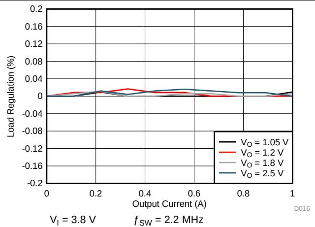
Figure 6-12. SMPS Load Regulation for 1-A Single Phase
