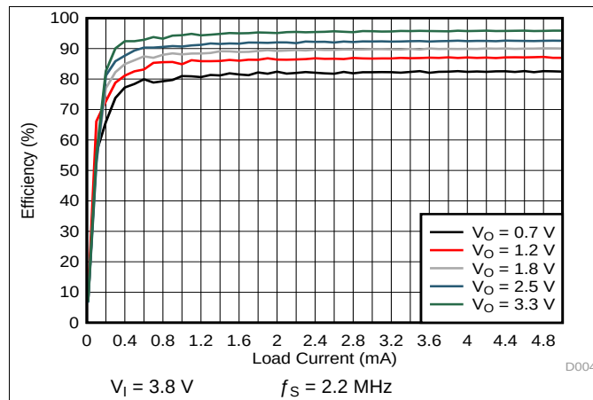
Figure 4-10. SMPS Efficiency for 2-A Single-Phase Eco-mode
