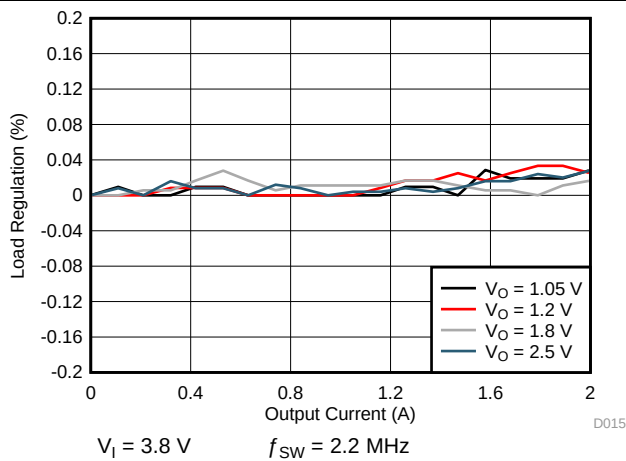
Figure 6-11. SMPS Regulation for 2-A Single Phase
