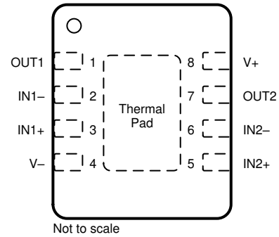
Figure 5-3. OPA2990 DSG Package (1) 8-Pin WSON With Exposed Thermal Pad Top View
