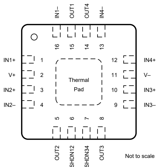
Figure 5-9. OPA4990S RTE Package (1) 16-Pin WQFN With Exposed Thermal Pad Top View
