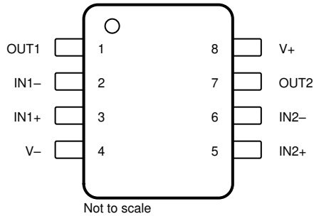
Figure 5-2. OPA2990 D, DDF, DGK, PW, and TDDF Packages (1) 8-Pin SOIC, SOT-23-8, TSSOP, and VSSOP Top View
