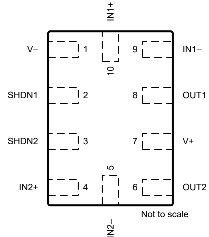
Figure 5-5. OPA2990S RUG Package 10-Pin X2QFN Top View
