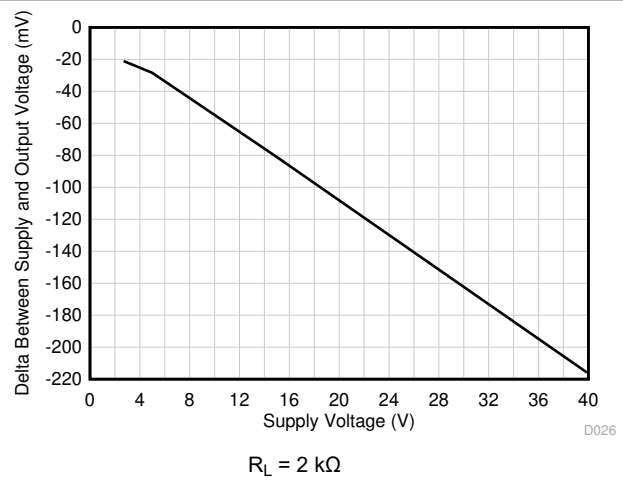
Figure 6-30. Output Swing vs Supply Voltage, Negative Swing
