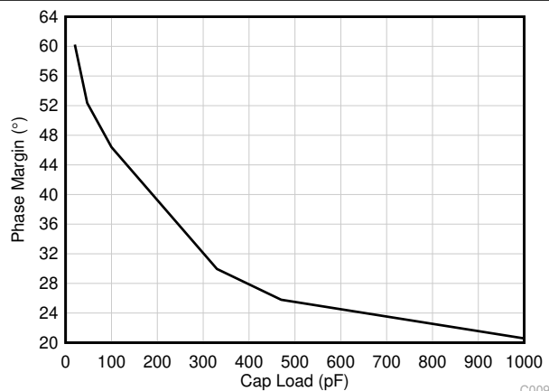
Figure 6-35. Phase Margin vs Capacitive Load
