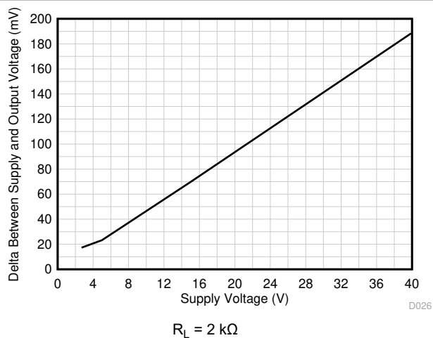
Figure 6-29. Output Swing vs Supply Voltage, Positive Swing
