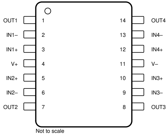
Figure 5-6. OPA4990 D and PW Packages 14-Pin SOIC and TSSOP Top View
