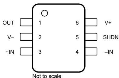
Figure 5-1. OPA990S DBV and DRL Package (1) 6-Pin SOT-23 and SOT-563 Top View
