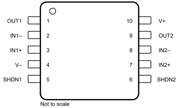
Figure 5-4. OPA2990S DGS Package 10-Pin VSSOP Top View
