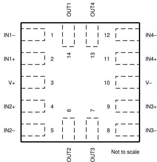
Figure 5-8. OPA4990 RUC Packages 14-Pin X2QFN With Exposed Thermal Pad Top View
