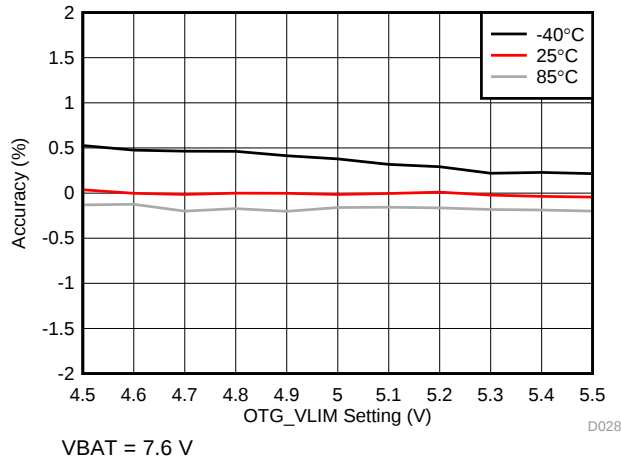
Figure 7. OTG VBUS Regulation vs OTG_VLIM Setting
