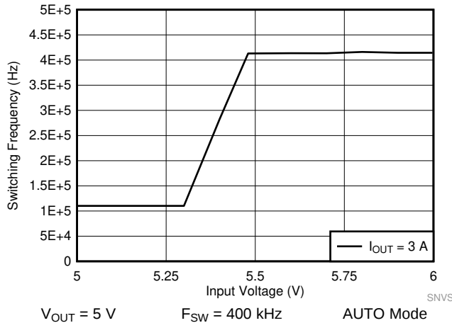
Figure 52. LM61440-Q1 Frequency Dropout Curve
