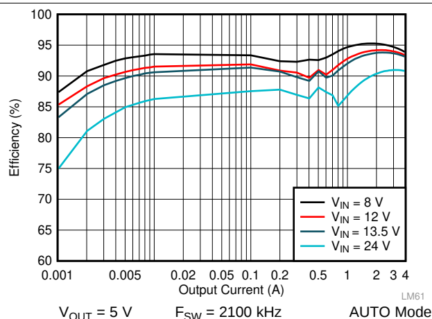
Figure 36. LM61440-Q1 Efficiency
