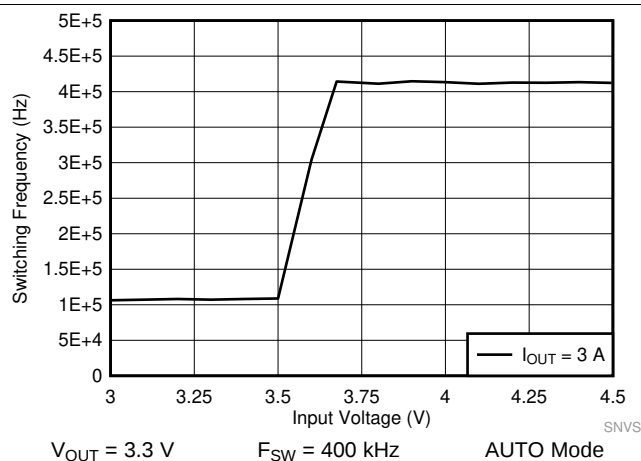
Figure 50. LM61440-Q1 Frequency Dropout Curve
