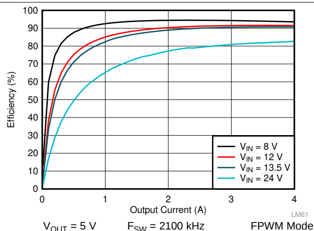
Figure 37. LM61440-Q1 Efficiency
