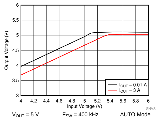
Figure 48. LM61440-Q1 Dropout Curve
