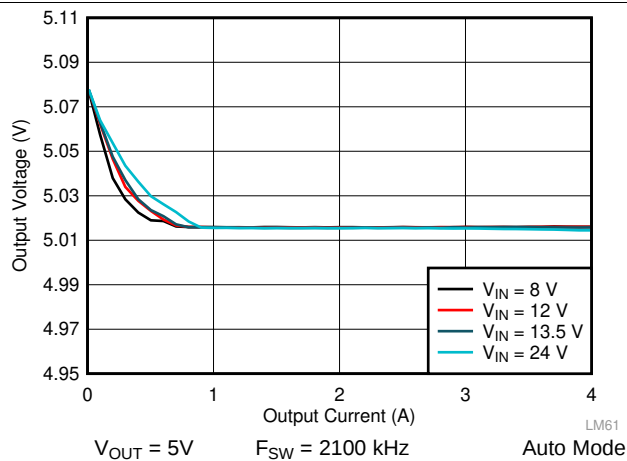
Figure 44. LM61440-Q1 Load and Line Regulation
