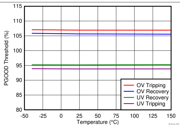
Figure 8. PGOOD Thresholds
