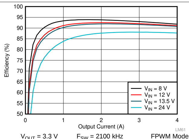
Figure 35. LM61440-Q1 Efficiency
