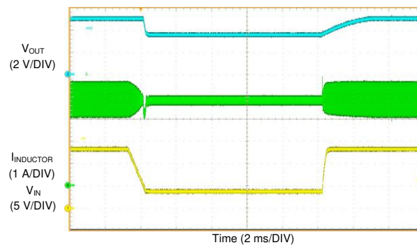
Figure 18. Recovery From Dropout ( V_{OUT} = 5\text{ V} , I_{OUT} = 4\text{ A} , V_{IN} = 13.5\text{ V} to 4\text{ V} to 13.5\text{ V} )
