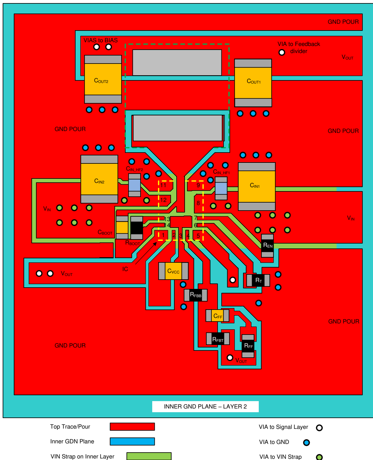
Figure 75. Layout Example
