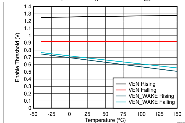
Figure 7. Enable Thresholds
