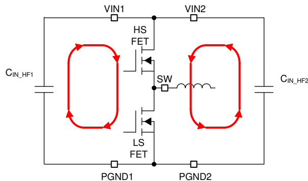
Figure 74. Input Current Loop
