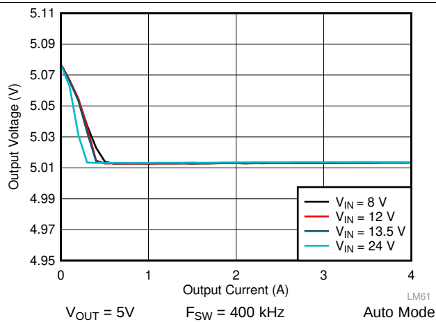
Figure 42. LM61440-Q1 Load and Line Regulation
