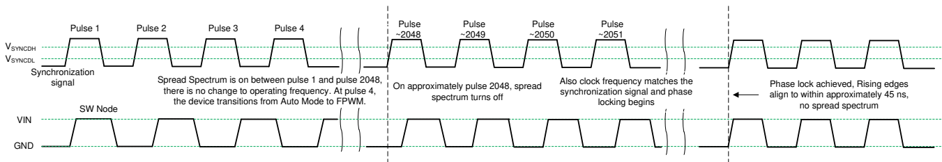
Figure 12. Synchronization Process
