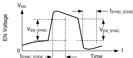
Figure 11. Typical SYNC/EN Waveform
