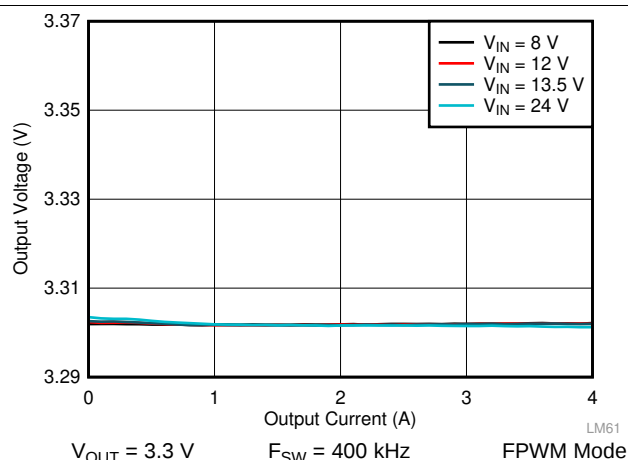
Figure 39. LM61440-Q1 Load and Line Regulation
