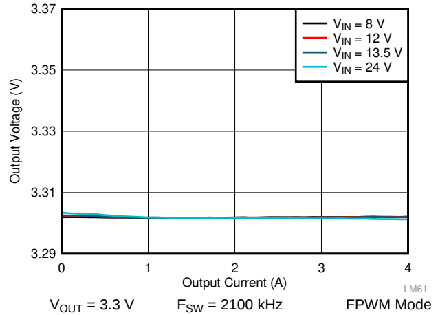
Figure 41. LM61440-Q1 Load and Line Regulation
