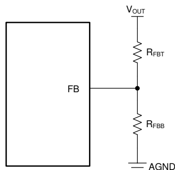
Figure 19. Setting Output Voltage of Adjustable Versions
