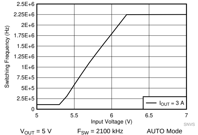
Figure 53. LM61440-Q1 Frequency Dropout Curve
