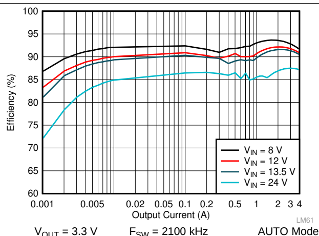
Figure 34. LM61440-Q1 Efficiency
