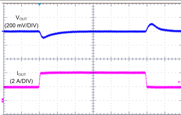
V_{OUT} = 3.3\text{ V} F_{SW} = 400\text{ kHz} AUTO Mode I_{OUT} = 2\text{ A to } 4\text{ A to } 2\text{ A} V_{IN} = 13.5\text{ V} T_R = T_F = 2\mu\text{s}
