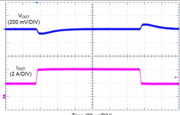
V_{OUT} = 3.3\text{ V} F_{SW} = 2100\text{ kHz} AUTO Mode I_{OUT} = 2\text{ A to } 4\text{ A to } 2\text{ A} V_{IN} = 13.5\text{ V} T_R = T_F = 2\mu\text{s}
