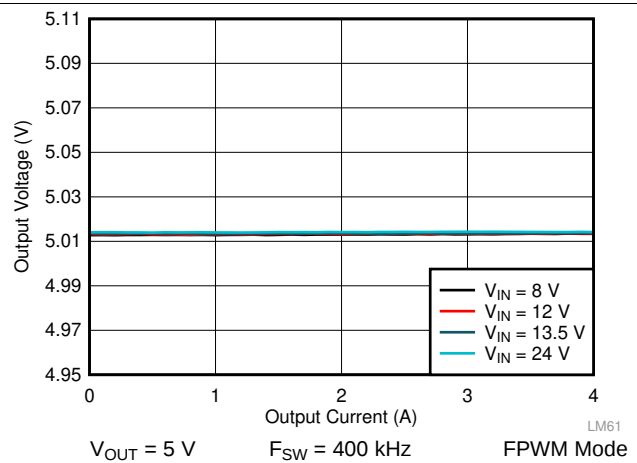
Figure 43. LM61440-Q1 Load and Line Regulation
