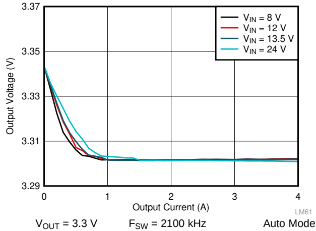
Figure 40. LM61440-Q1 Load and Line Regulation
