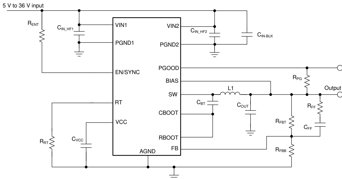
Figure 30. Example Application Circuit
