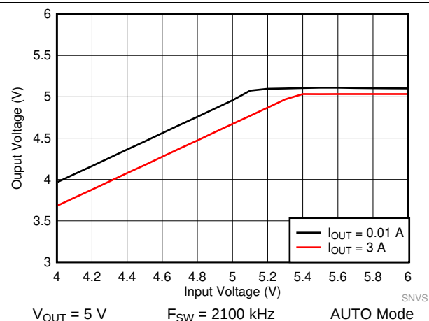
Figure 49. LM61440-Q1 Dropout Curve
