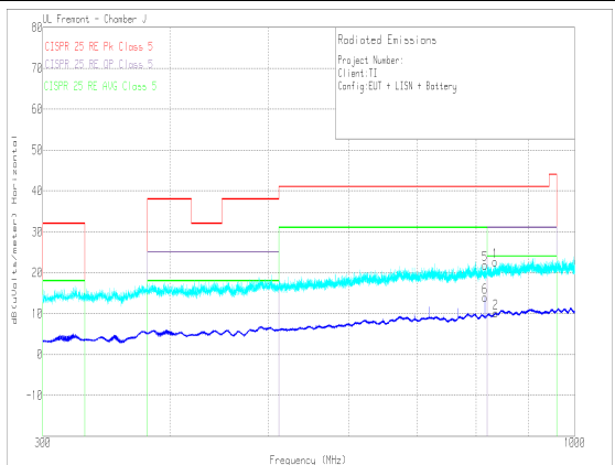
Figure 67. Radiated EMI Bicon Horizontal versus CISPR25 Limits
