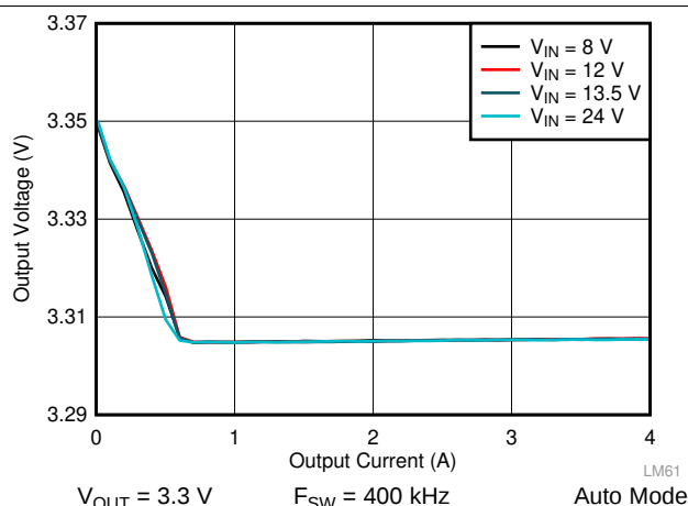
Figure 38. LM61440-Q1 Load and Line Regulation
