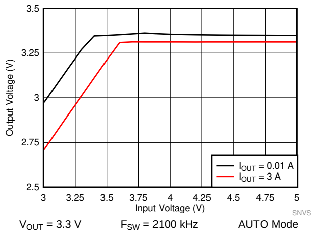
Figure 47. LM61440-Q1 Dropout Curve
