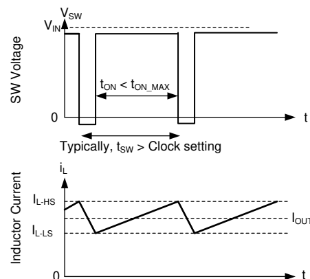
Figure 20. Current Limit Waveforms
