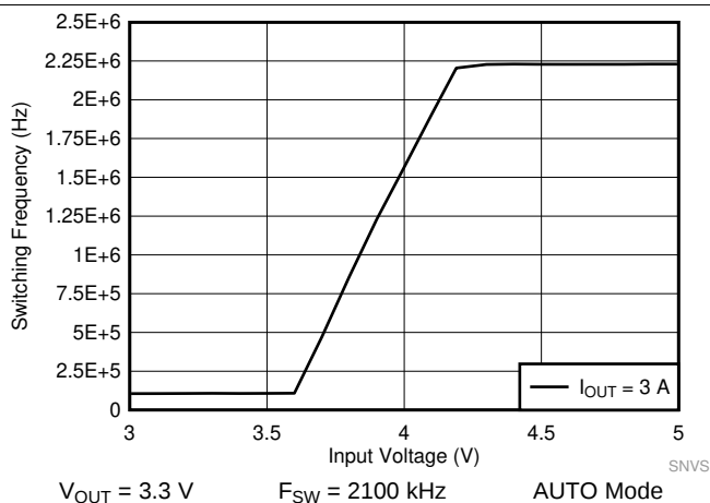
Figure 51. LM61440-Q1 Frequency Dropout Curve
