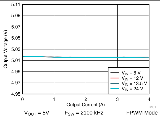
Figure 45. LM61440-Q1 Load and Line Regulation
