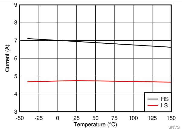
Figure 4. LM61440-Q1 High-side and Low-side Current Limits
