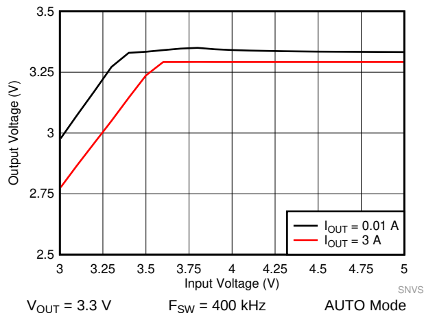
Figure 46. LM61440-Q1 Dropout Curve
