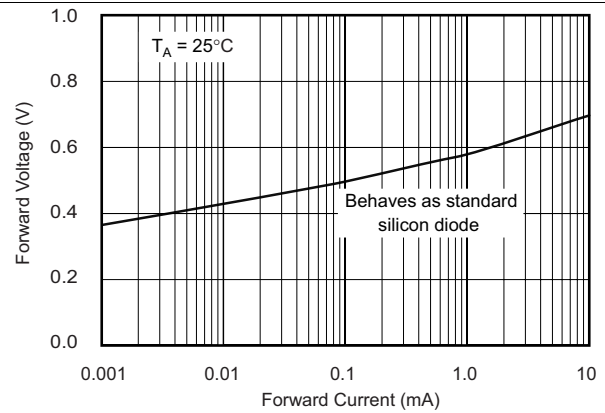
Figure 2. Forward Characteristics
