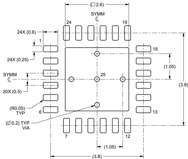
LAND PATTERN EXAMPLE SCALE:15X
