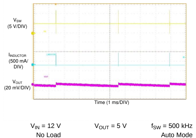
Figure 58. LM76003 Switching Waveform and Output Ripple
