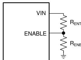
Figure 12. V_{IN} UVLO
