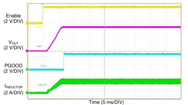
Figure 67. Start-up Waveform
