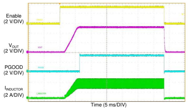
Figure 65. LM76003 Start-up Waveform
