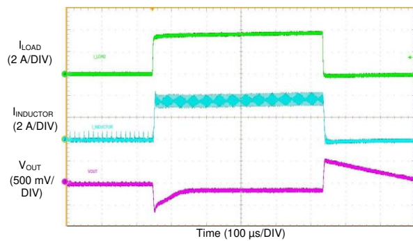
Figure 79. LM76003 Load Transient
