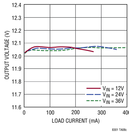
Output Load and Line Regulation
