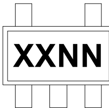
5-Lead SOT-23 (MCP6H01)
